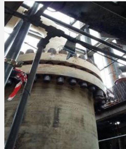
Fully boxed-up boiler c/w Cover Channel and interconnecting piping.
